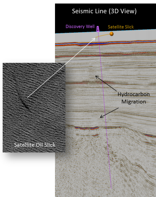
Figure 2. Satellite oil slick imaged over known oil discovery offshore Newfoundland and Labrador.
