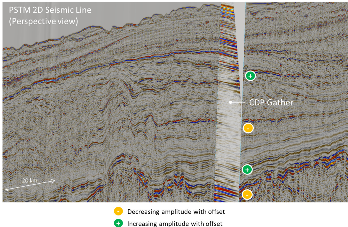
Figure 4. Perspective view of a 2012 deepwater Labrador Sea seismic line showing a broad Eocene aged structure and a CDP gather showing Class III AVO behavior in the upper portion of the structure.
