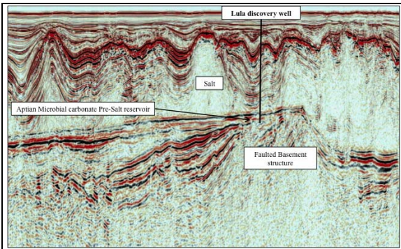
Figure 2: Seismic line across the Lula Field (depth-migrated dual-sensor streamer 2D line)
