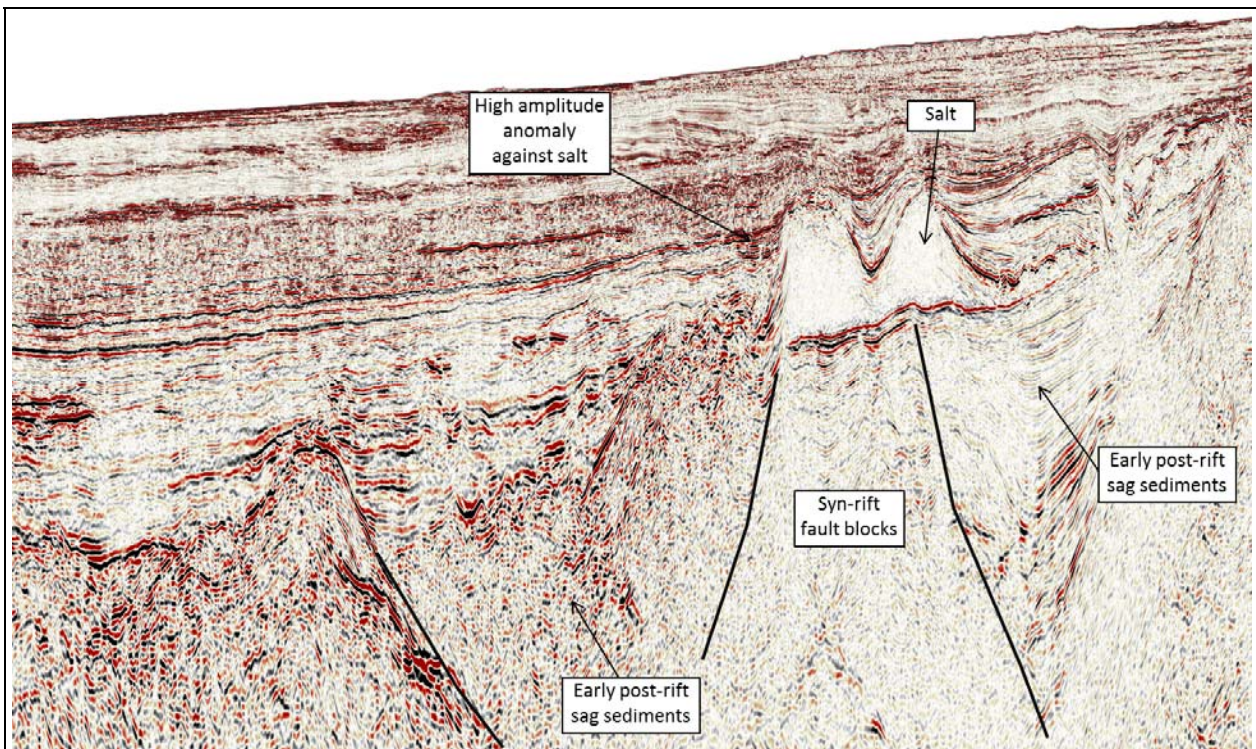
Figure 3. Dual-sensor streamer 2D dip line over the Namibe Basin (interim depth-migrated, 2011).
