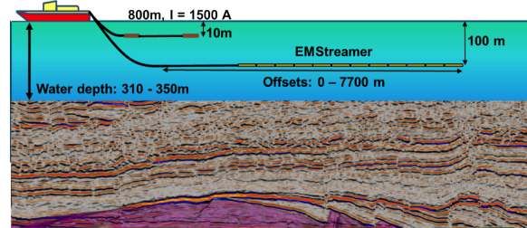
Figure 1. The Towed Streamer EM System configuration.
