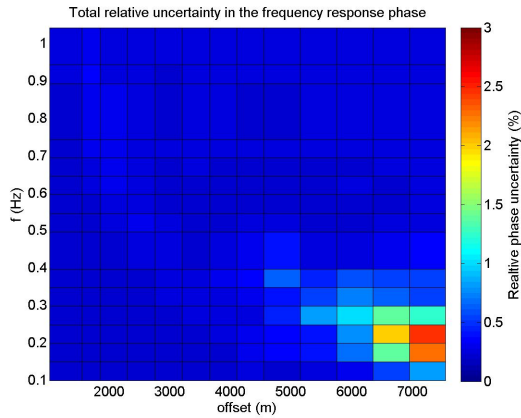
Figure 3. The total relative uncertainty in the frequency response phase for one of the survey lines at the TWOP field.
