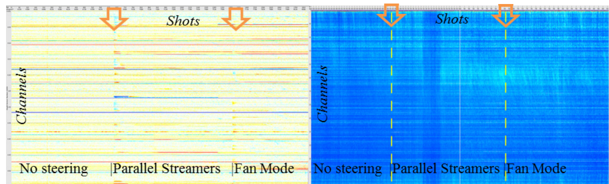
Figure 4 Single Sailline: Left: streamer depth, Right: RMS noise plot. For each shot (x- axis), the depth or RMS noise is plotted in colour for each receiver (y- axis), arrows mark the shot where the steering mode was changed.
