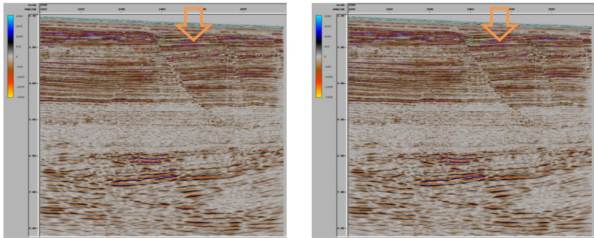
Figure 2 Example from the decimation tests performed on legacy 3D data. The section to the left shows a crossline stack with no holes in the coverage. In the right section, a coverage hole of 180m has been introduced at the far-mid offset range.
