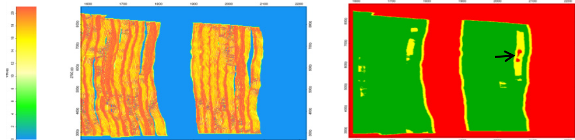
Figure 3 Left: the fold achieved at the far offset interval. Right: the acceptability plot. The red area on the acceptability plot (arrowed) highlights where additional infill is needed to maintain image quality.
