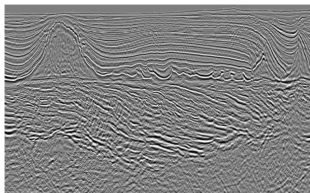
Figure 7: TTI RTM (35 Hz). Note the steeply dipping reflectors (SDRs)
