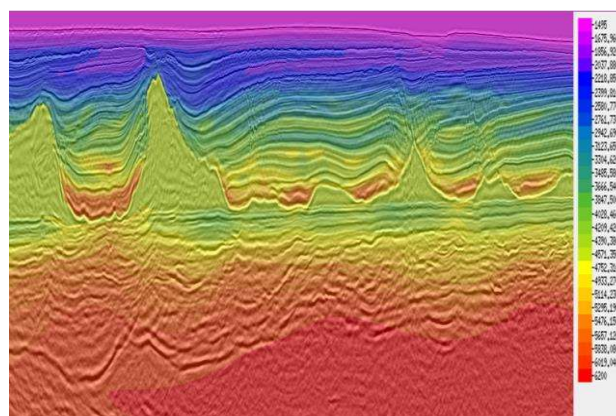
Figure 4: TTI RTM overlaying the velocity model. The presalt events exhibit good continuity
