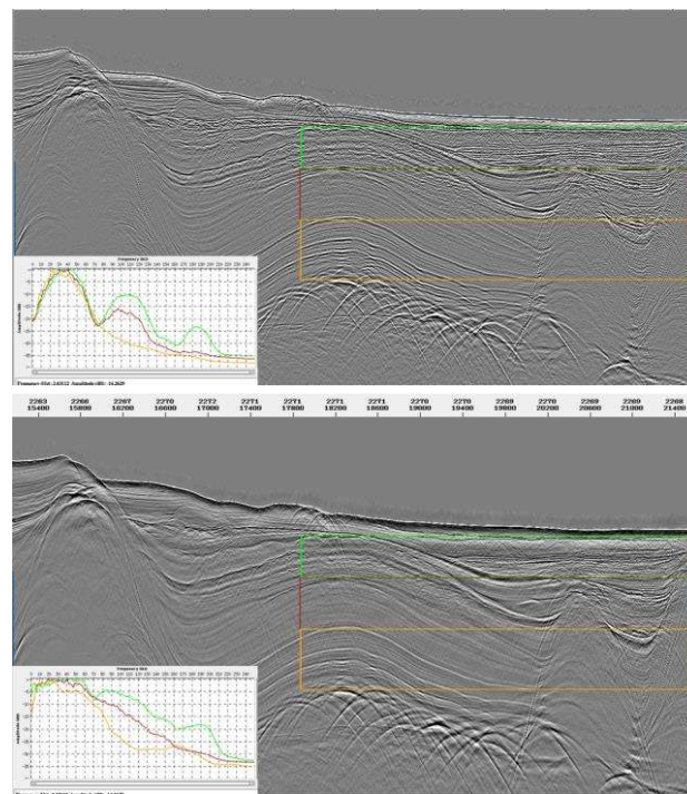
Figure 3: Stack from Campos Basin Before (Top) and After De-Ghosting (Bottom).
